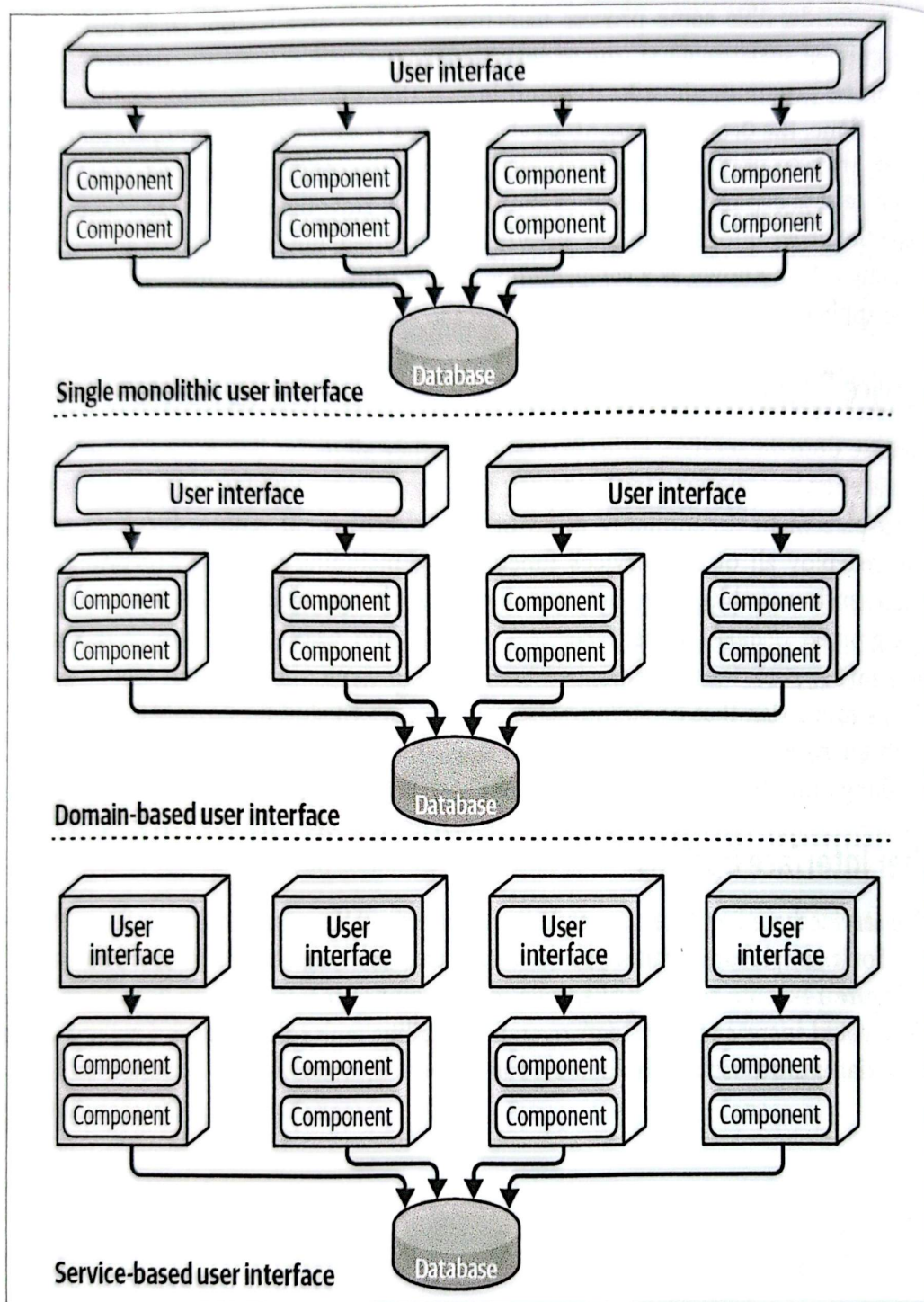
Figure 14-3. Three user-interface variants in a service-based architecture
