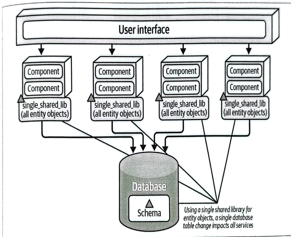
Figure 14-6. Using a single shared library for database entity objects impacts all services when a change occurs and is considered an antipattern in service-based architecture
