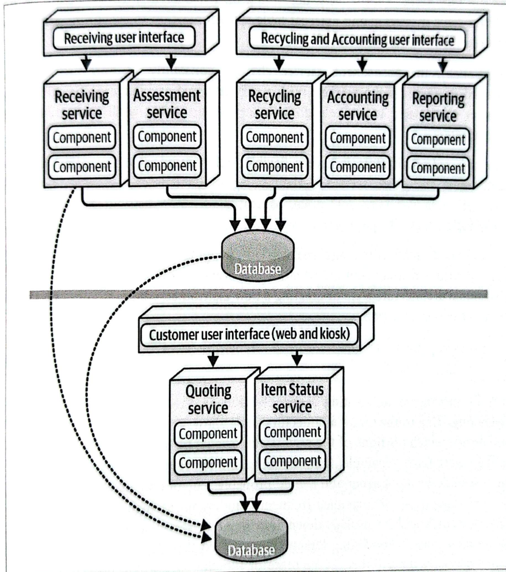
Figure 14-10. Going Green's electronics recycling application using service-based architecture
